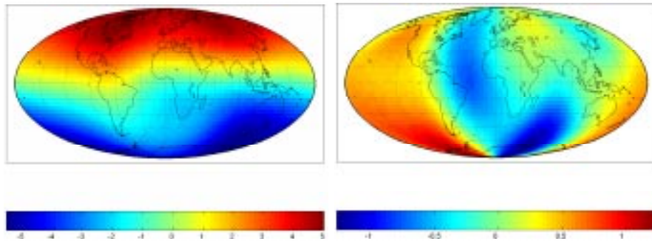
Figure 12: Denoised -\varepsilon^r -component (left) and \varepsilon^\varphi -component in 10000 [nT]
