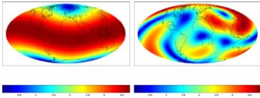
Figure 15: Toroidal Intensity at scales 0 (left) and 1 (right); [nT]
