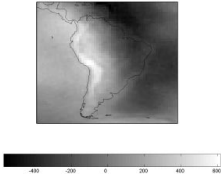
Figure 4: Denoised graviational potential over South America [100 Gal m]
