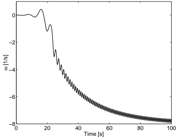
Figure 5: The angular velocity of a non-perfect permanent magnet in a non-homogeneous temperature field. y_0^m = 5 \cdot 10^{-7}[\text{m}]
