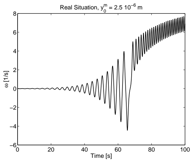
Figure 7: The angular velocity of a non-perfect permanent magnet in a non-homogeneous temperature field. y_0^m = 2.5 \cdot 10^{-6} [m]
