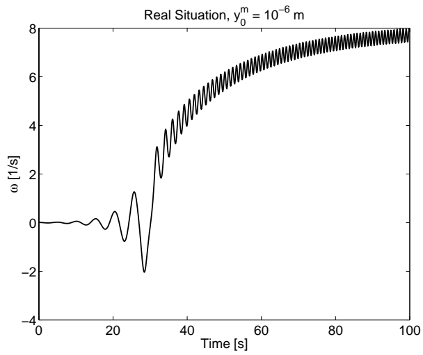
Figure 6: The angular velocity of a non-perfect permanent magnet in a non-homogeneous temperature field. y_0^m = \cdot 10^{-6}[\text{m}]
