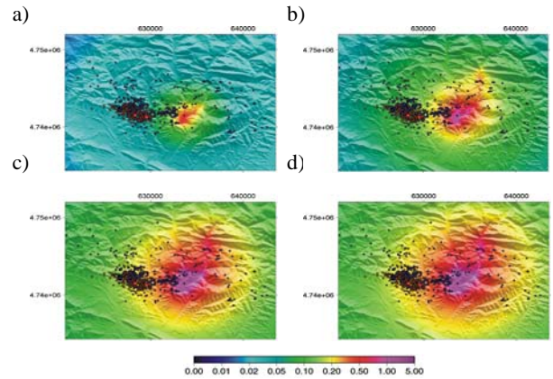
Figure 12. Vertical surface elastic displacements due to water loads (cm). a) 18/09/2004 (earthquake mainshock, Mw=4.7); b) 01/06/2006, c) 01/07/2007, d) 18/04/2008 (maximum capacity), (see [1]).
