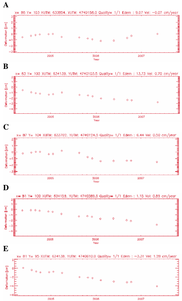
Figure 8. Time series of A-E pixels. ENVISAT data dates.
