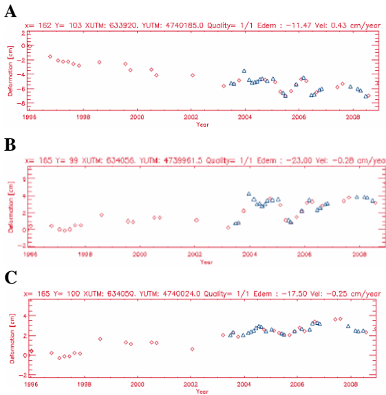
Figure 5. Time series of A-C pixels. ERS data dates in red. ENVISAT data dates in blue.
