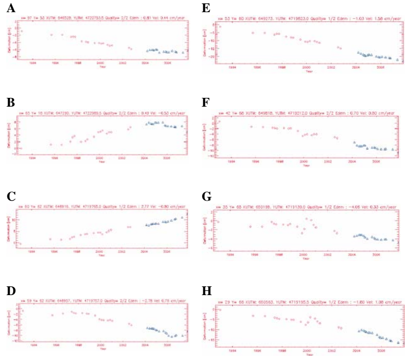
Figure 11. Time series of A-E pixels. ERS data dates in red. ENVISAT data dates in blue.
