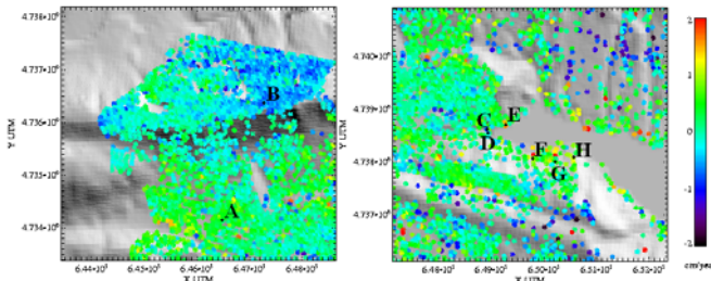
Figure 10. Deformation map of two interesting areas of Yesa. Darker colour means positive and softer colour means negative LOS velocity of displacements.
